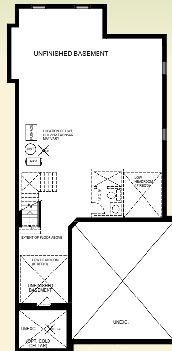
Basement Plan Elev. A
