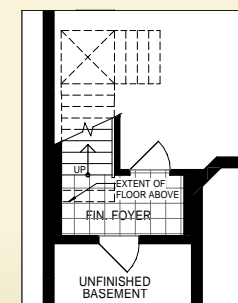
Partial Basement Plan w/ Opt. Finished Stairs Elev. A
