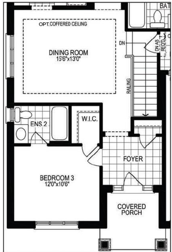
PART. GROUND FLOOR PLAN W/ OPT. 3 BEDROOM LAYOUT, EL. 'A'
