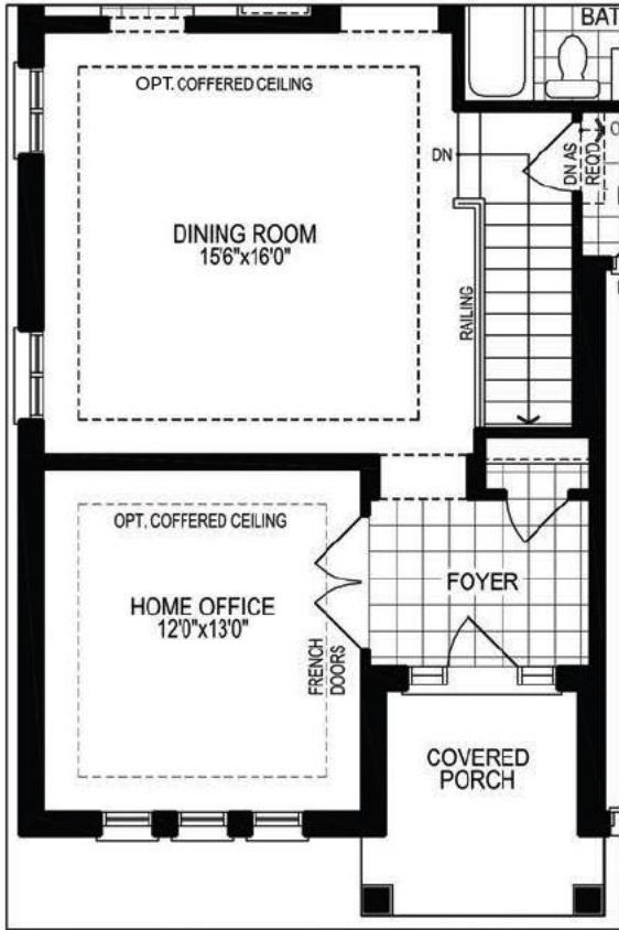
PART. GROUND FLOOR PLAN W/ OPT. HOME OFFICE LAYOUT, EL. 'B'
