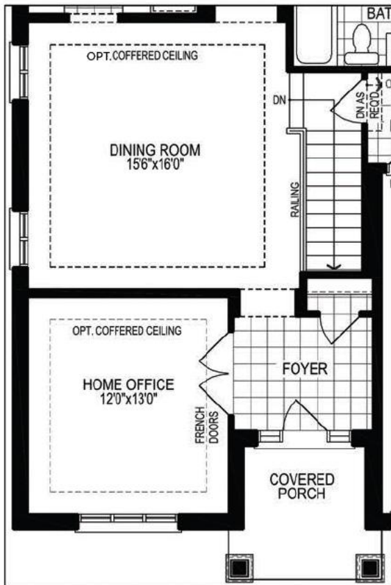
PART. GROUND FLOOR PLAN W/ OPT. HOME OFFICE LAYOUT, EL. 'A'
