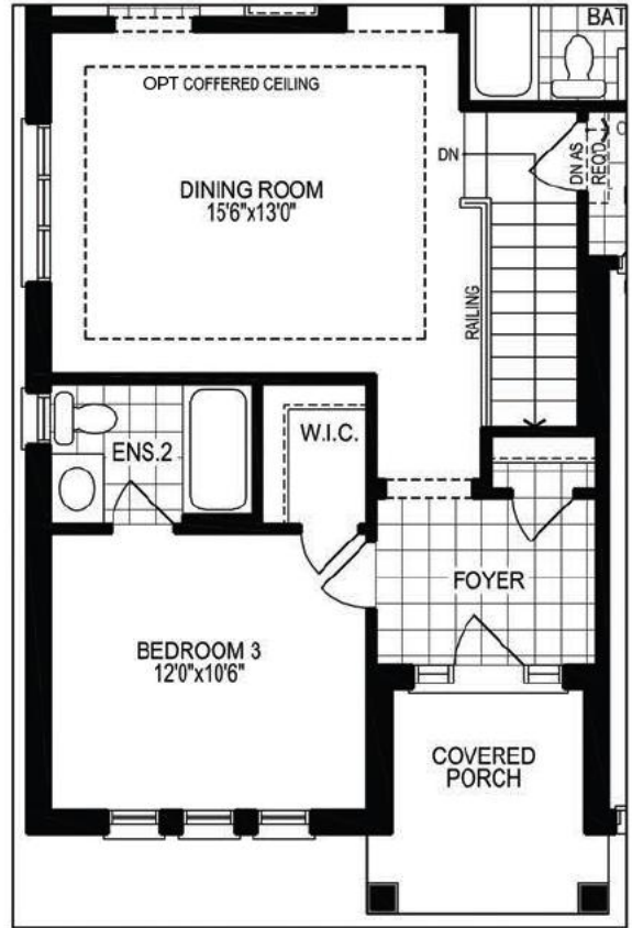
PART. GROUND FLOOR PLAN W/ OPT. 3 BEDROOM LAYOUT, EL. 'B'
