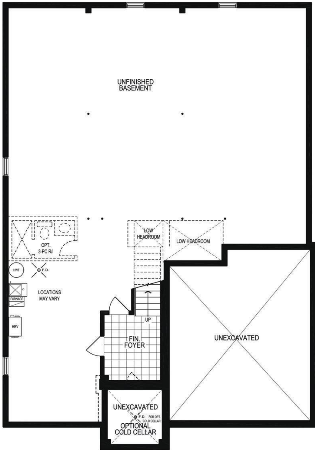
BASEMENT PLAN, EL. 'A'
